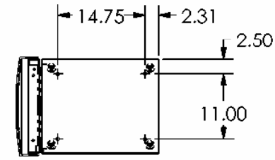
SECTION A-A ANCHOR DRILL TEMPLATE
